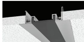
75FCA Acoustical Ceiling 1-2" [25-50mm] ±25% / Thermal
