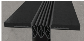
CS ● ● ● ● Winged Multi-chambered Seal 1.5-4" [37.5-100mm] Varied / Seismic Slow Vehicular
