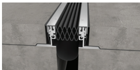
SSPD ● ● ● ● Split Slab Multi-chambered Seal 2.5-3.5" [62.5-87.5mm] ±50% / Seismic Pedestrian
