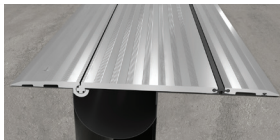
DFH ● ● ● ● Surface Mount Hinge 3-8" [75-200mm] ±50% / Seismic Slow Vehicular
