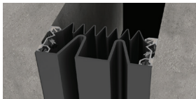
FCWW ● ● ● ● Flush Wall 2-18"+ [50-450mm+] ±50% / Seismic Santoprene or Silicone
