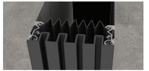
FCVS ● ● ● ● Flush Wall 2-18"+ [50-450mm+] ±100% / Seismic Santoprene or Silicone
