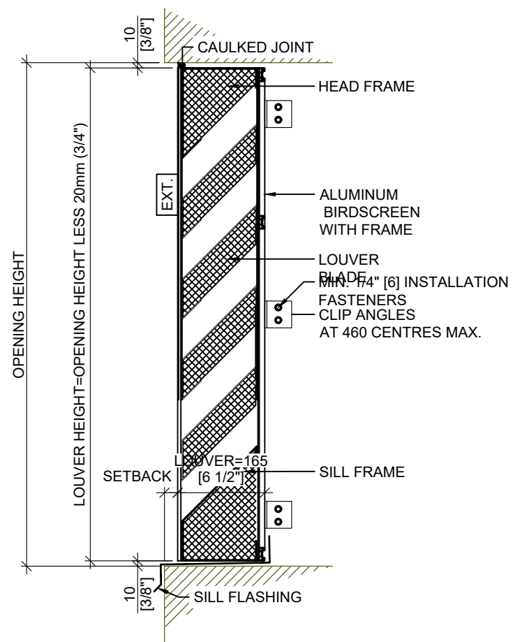
SECTION
