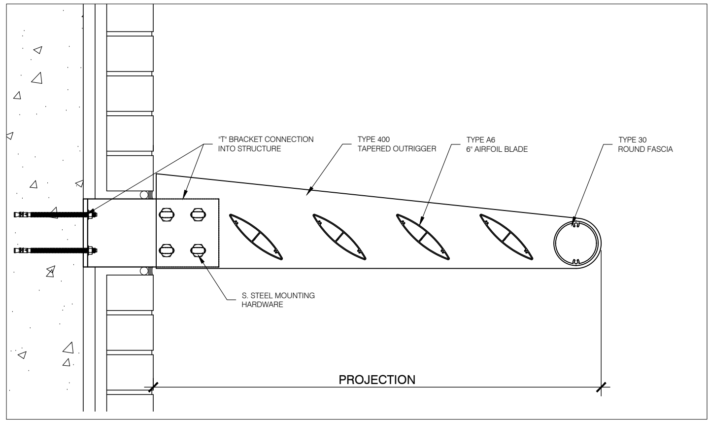
MODEL A6-400-30 CROSS SECTION
