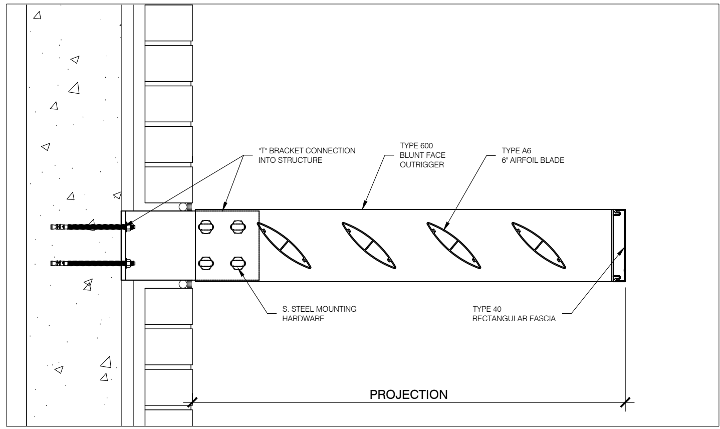
MODEL A6-200-40 CROSS SECTION
