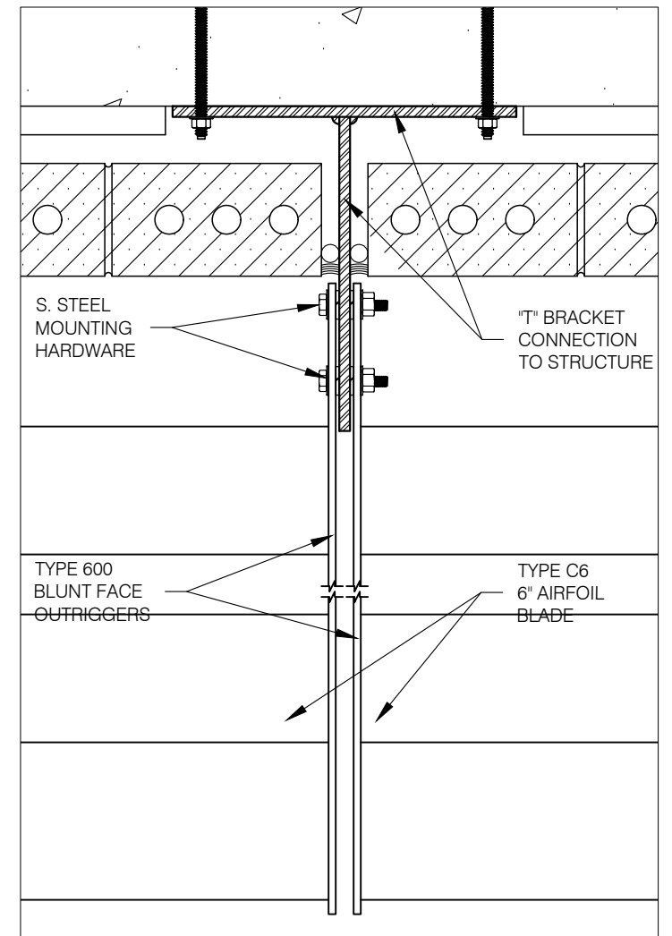
PLAN AT "T" BRACKET CONNECTION
