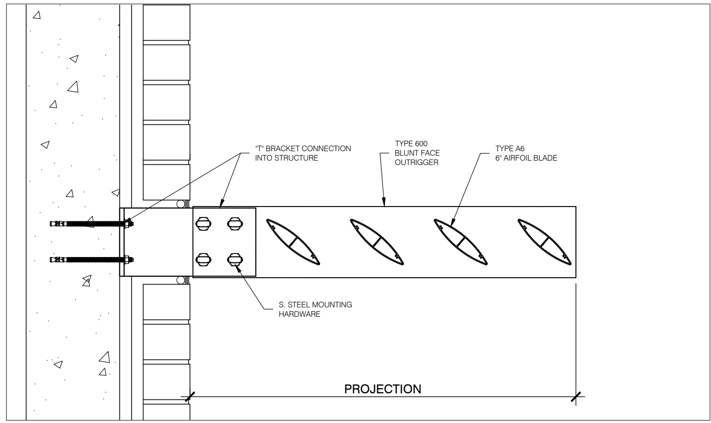
MODEL A6-200-10 CROSS SECTION
