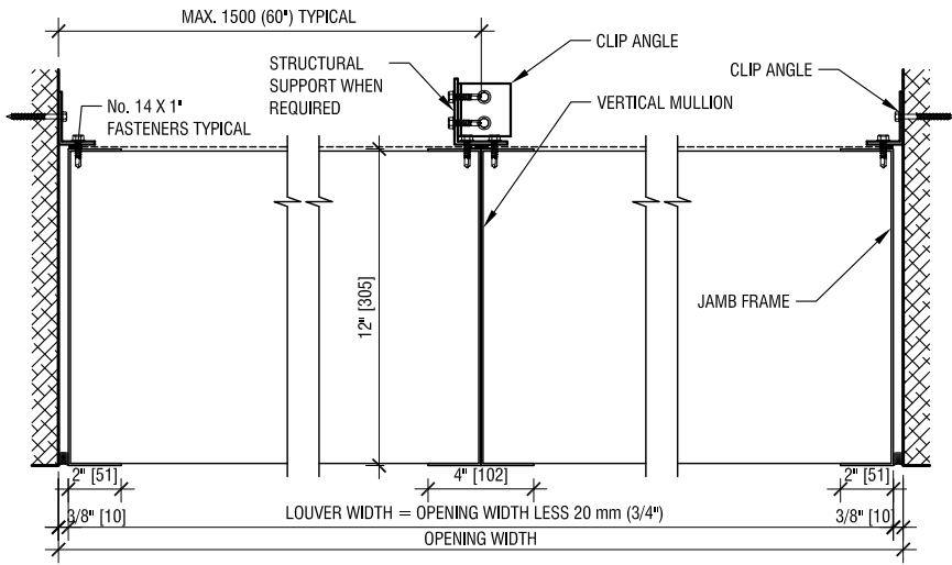
HORIZONTAL SECTION
